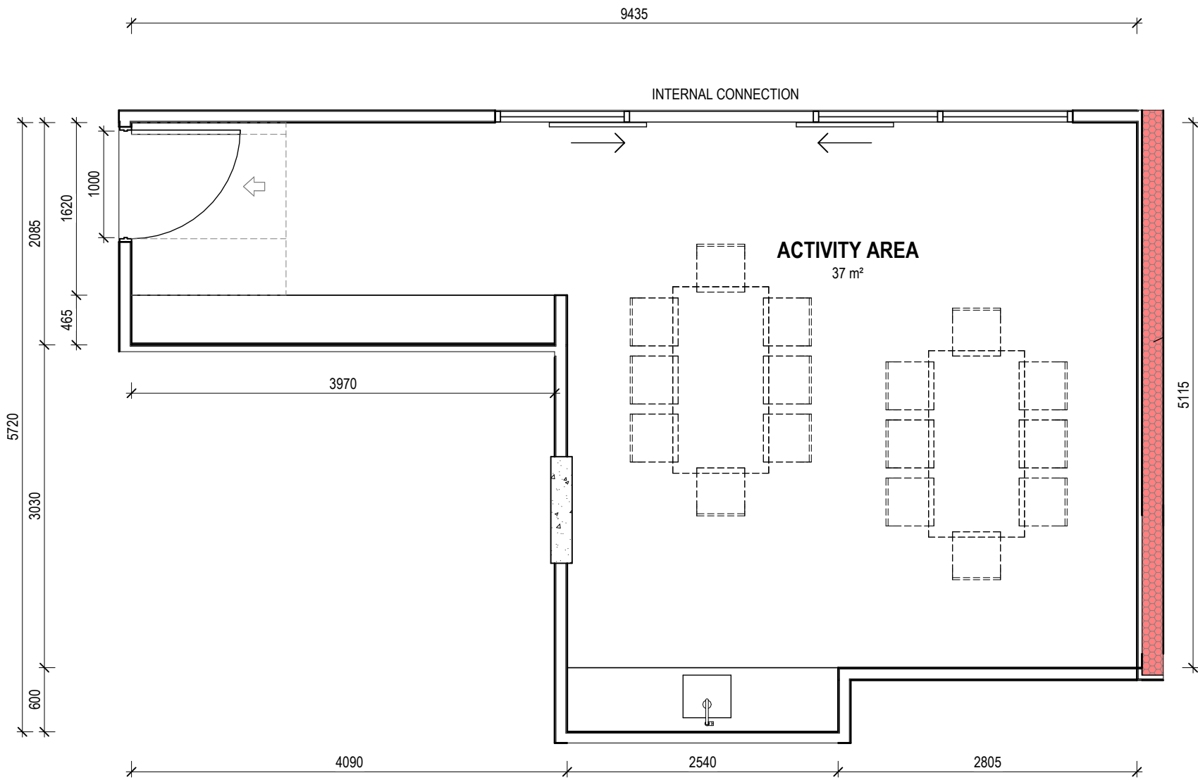
VILLAGE COMMUNAL - ACTIVITY AREA Scale 1 : 50
