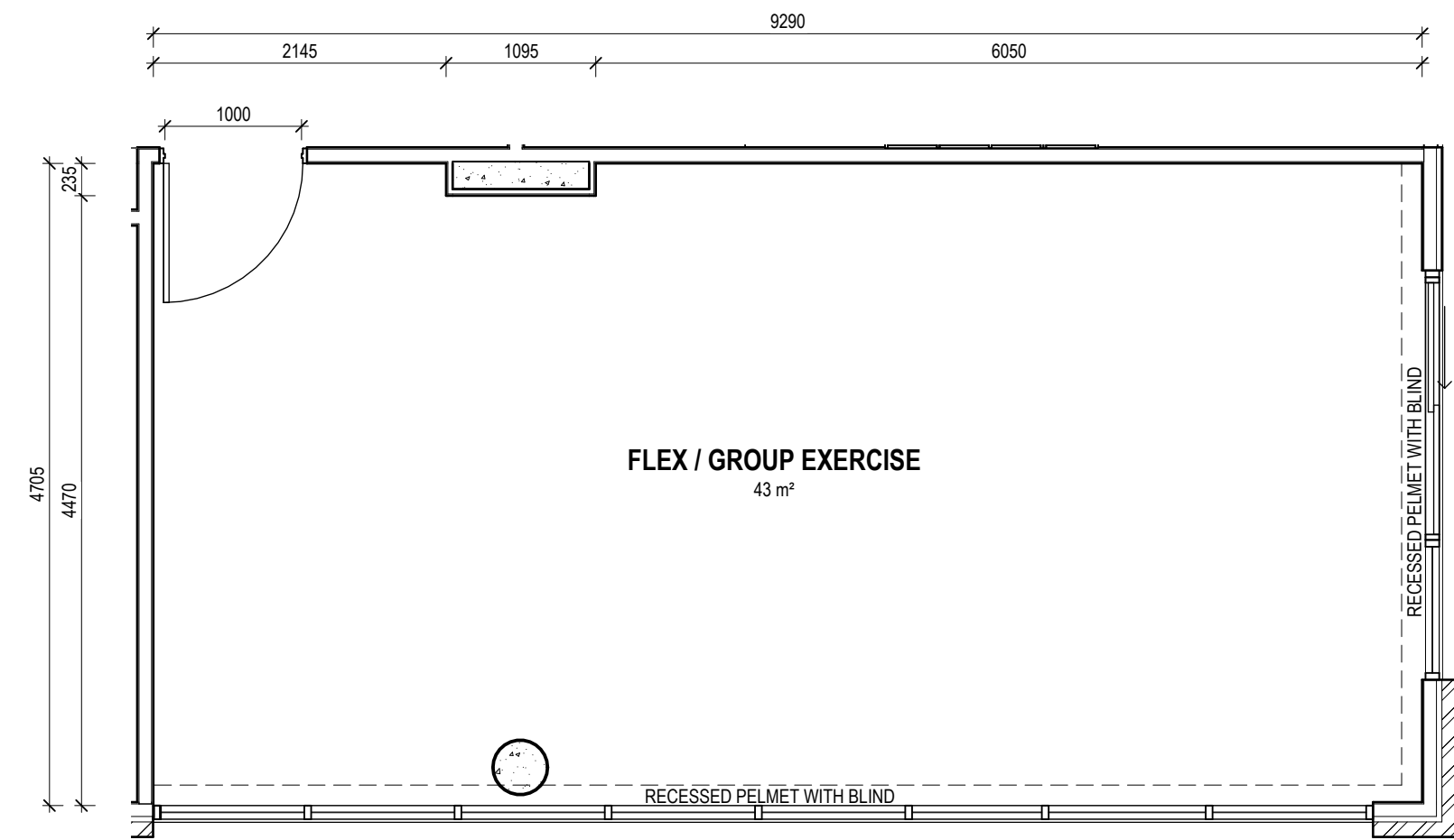
VILLAGE HEALTH & WELLNESS - FLEX/GROUP EXERCISE Scale 1 : 50
